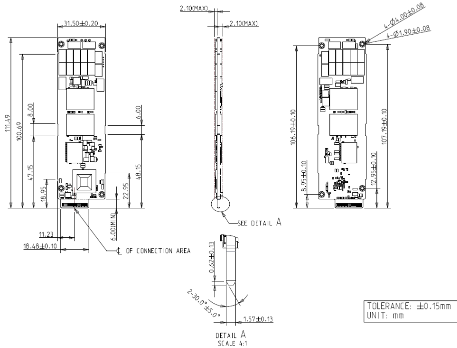
Diagram 5.9mm (6.4TB)
