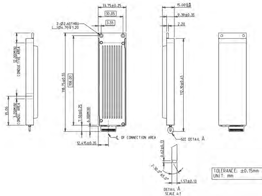
Diagram 15mm enclosure
