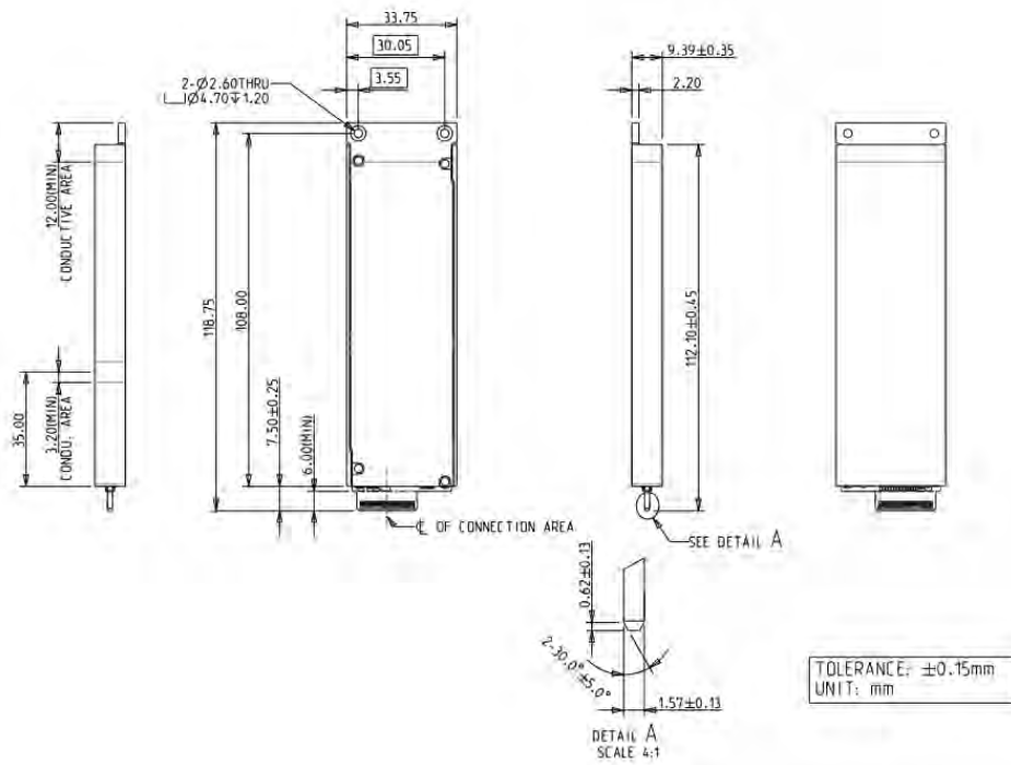
Diagram 9.5mm enclosure
