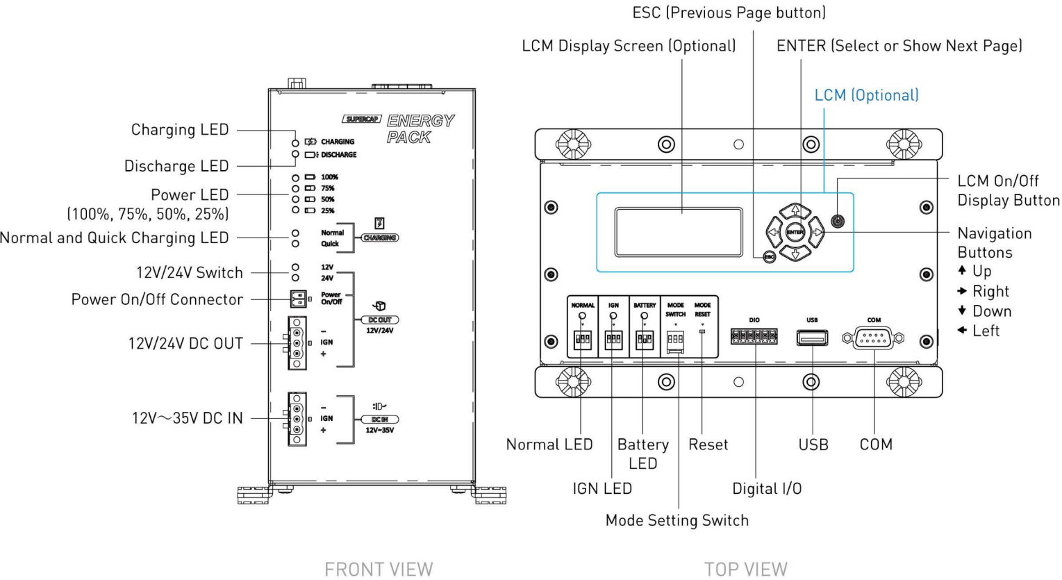
External I/O Mechanical Layout
