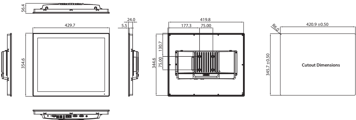
Panel Cutout Dimensions: 420.9 x 345.7 mm (16.57 x 13.61 in)
