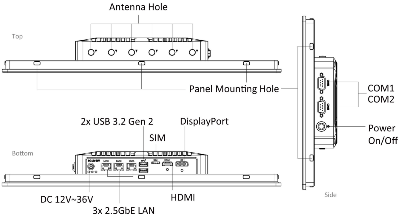
External I/O Mechanical Layout
